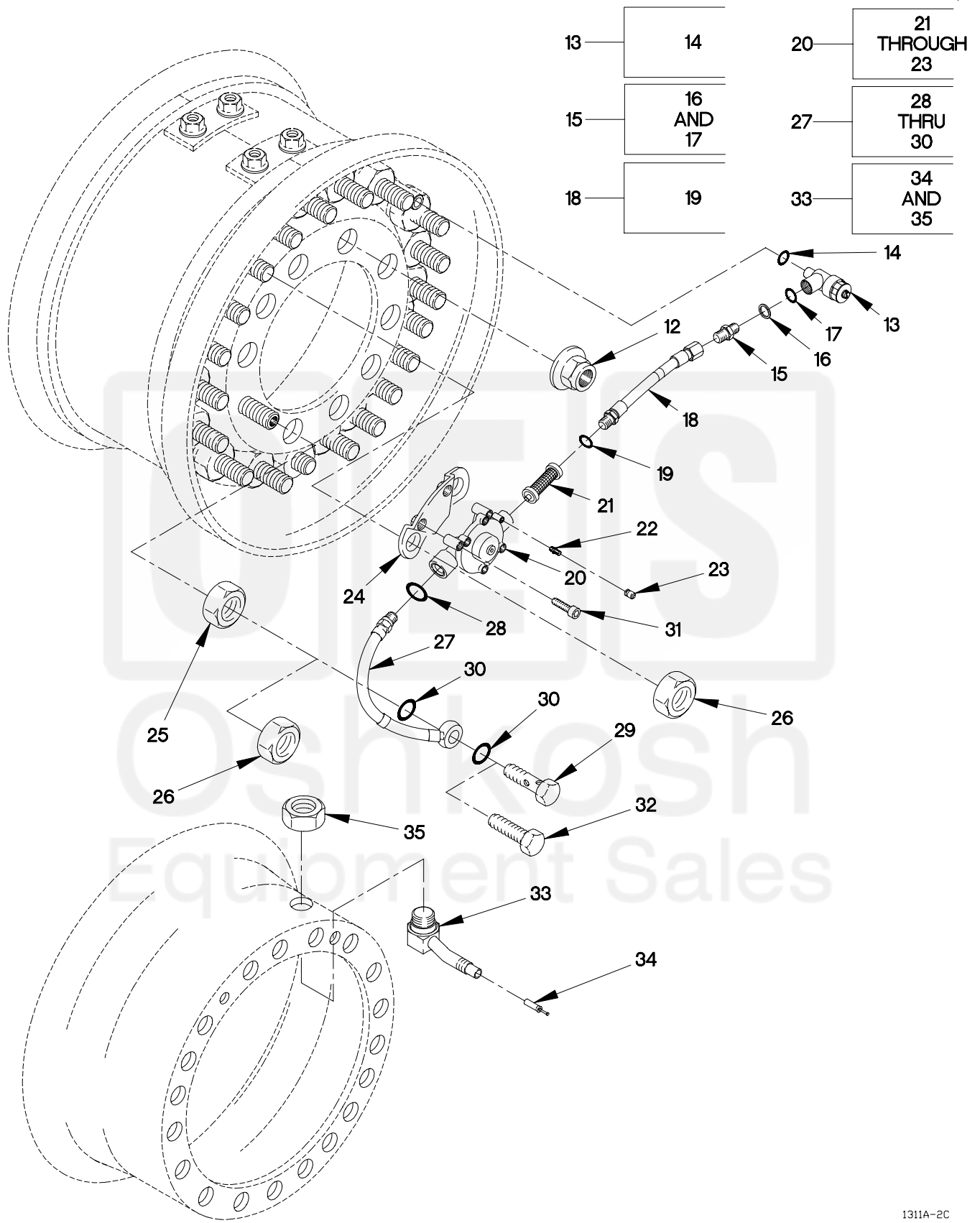
FIGURE 158. WHEEL ASSEMBLY AND CTIS VALVE (SHEET 2 OF 2)
